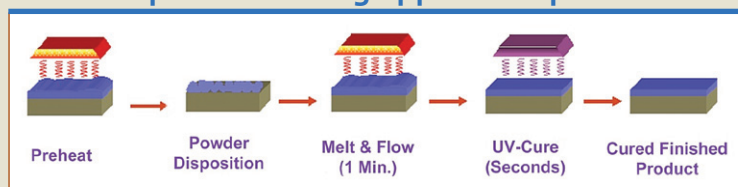
UV-cured powder coating application process
